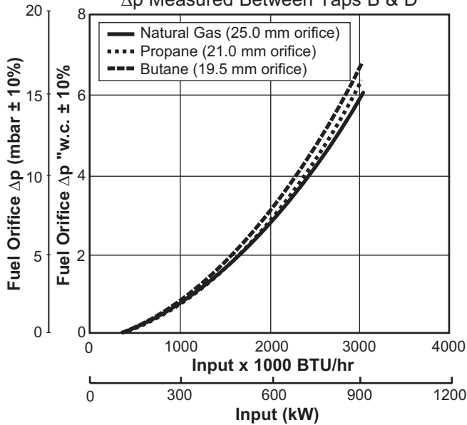
Fuel Orifice Δp vs. Input
